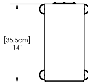
TOP VIEW (WITH GRILLE)
